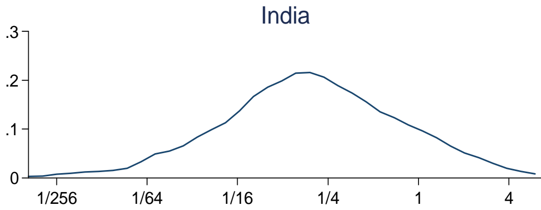
Figure 1: Distribution of TFPQ
